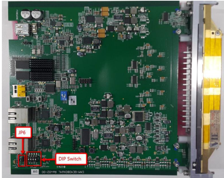
Figure 5 DIP Switch location
